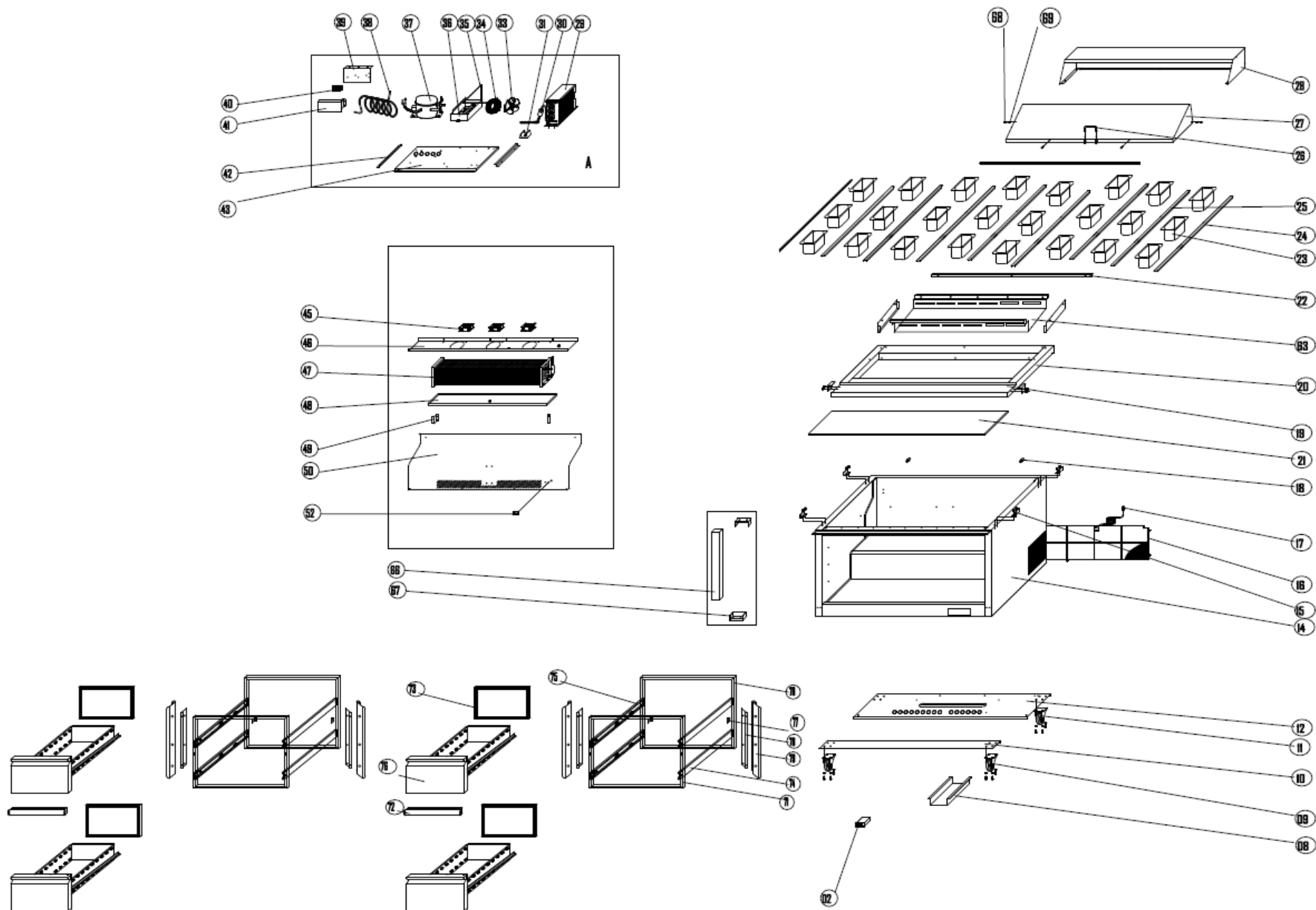
EXPLODE OF KCHMT60.24.4D
